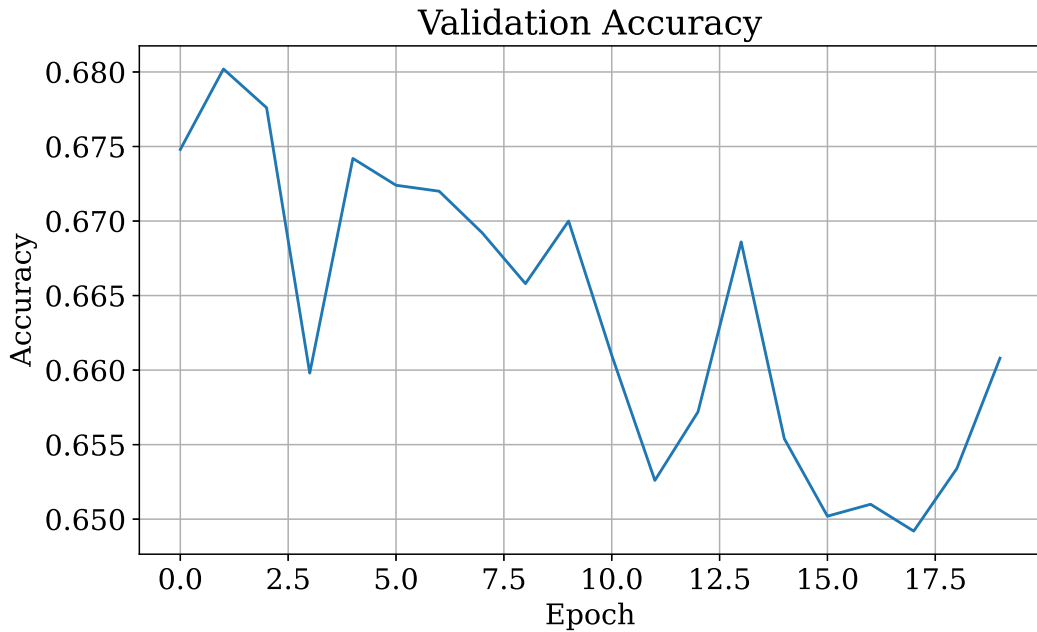
Figure 4: Validation accuracy over 20 epochs.
