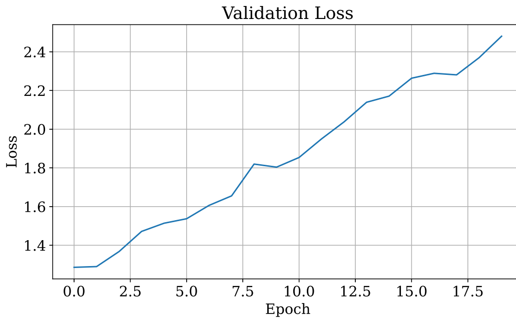
Figure 6: Validation loss over 20 epochs.
