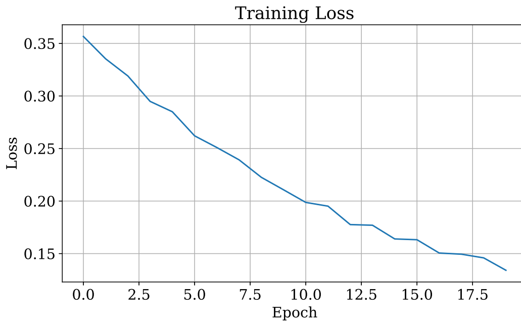
Figure 5: Training loss over 20 epochs.
