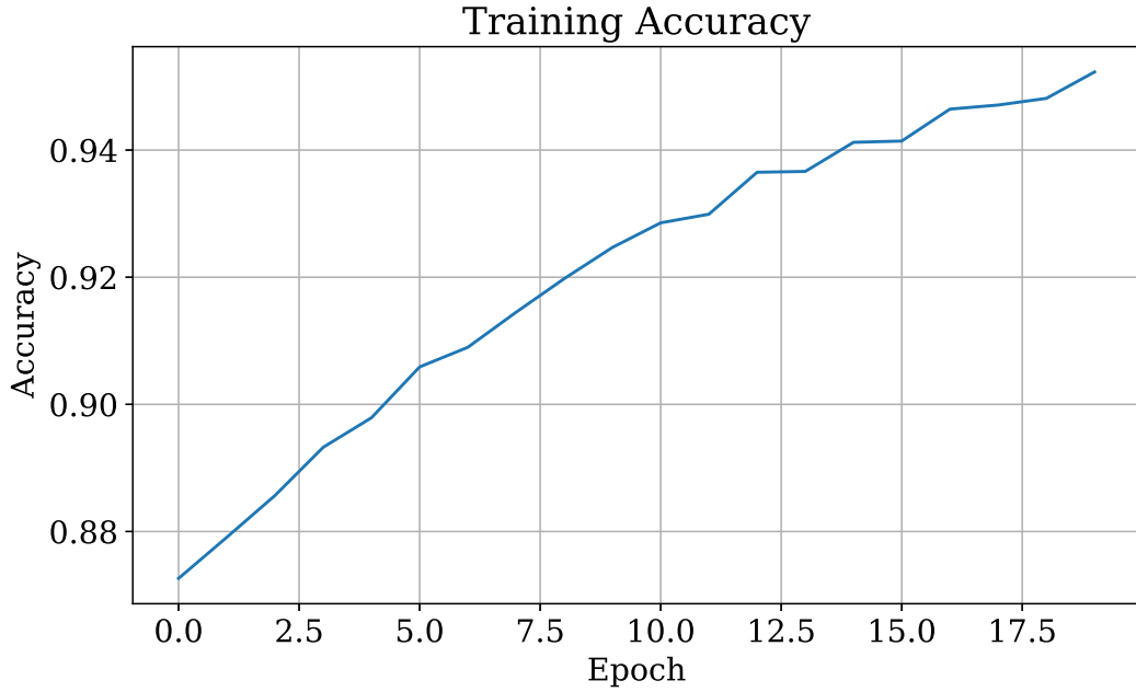
Figure 3: Training accuracy over 20 epochs.
